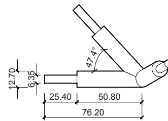
Joint Typical Detail
